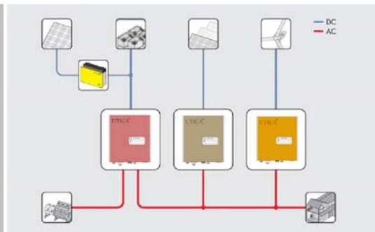
Off-grid System
