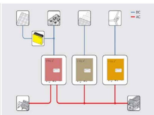
Off-grid System
