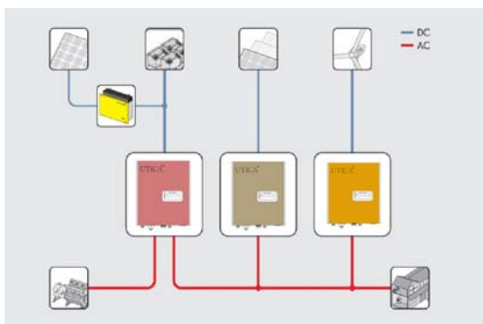
Off-grid System
