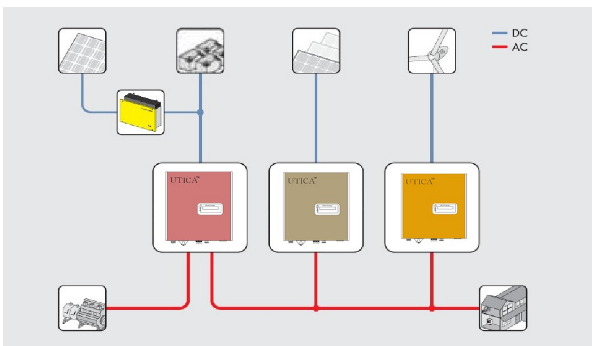
Solar Off-grid System
